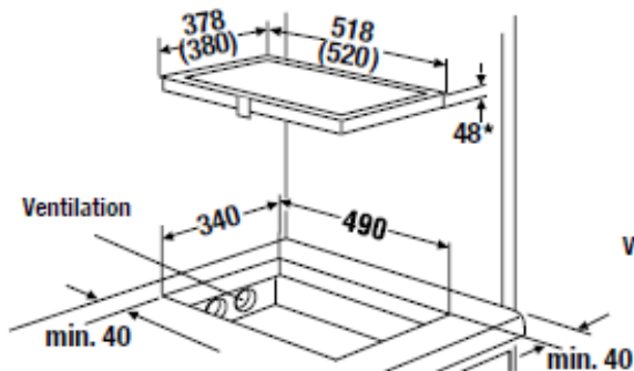
Top mount installation (with steel profiles)
